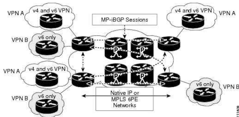
Figure 4-1 6VPE Deployment
